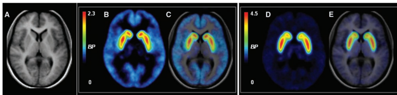
Fig. 1. Maps of baseline D1 and D2 BP, averaged across 13 human volunteers. (A) The averaged MRI, normalized to MNI space. (B) D1 BP, measured with [ 11 C]SCH23390, averaged across participants (the bar shows absolute D1 BP). (C) Overlay of (B) on (A). (D) D2 BP, measured with [ 11 C]Raclopride, averaged across participants (the bar shows absolute D2 BP). (E) Overlay of (D) on (A).
